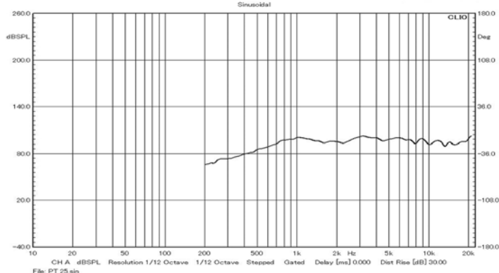
Frequency response curve (* This data was not measured in car.)
