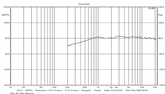
Frequency response curve (* This data was not measured in car.)
